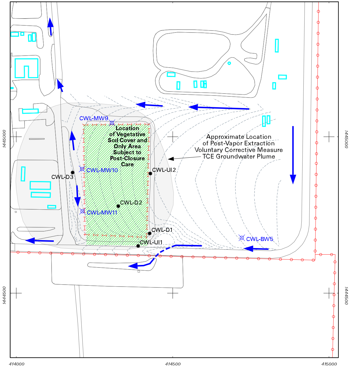
Figure 6 Site Layout for the Post-Closure Care Period Chemical Waste Landfill
