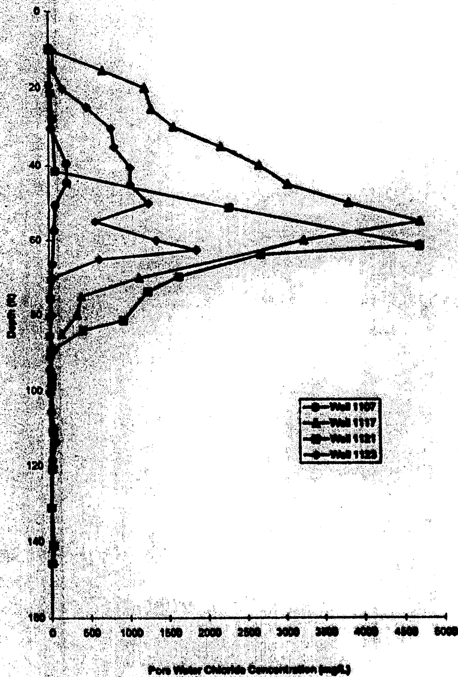
Figure 1. Chloride profiles for wells 1107, 1117, 1121, and 1123.
