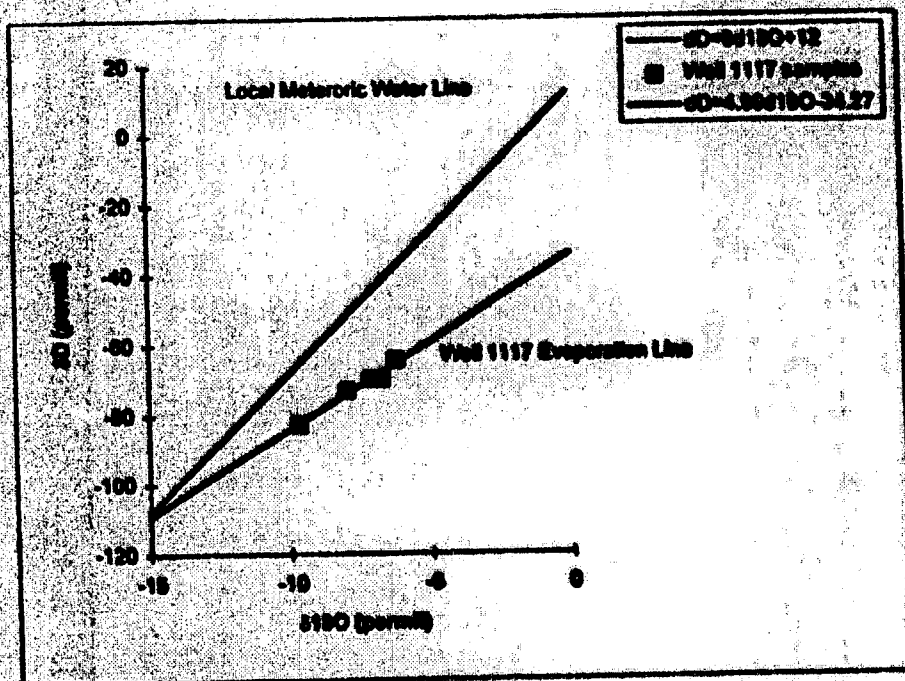
Figure 5. Meteoric water plot of well 1117 waters. The local meteoric water line is from Vustaz and Goff (1968).
