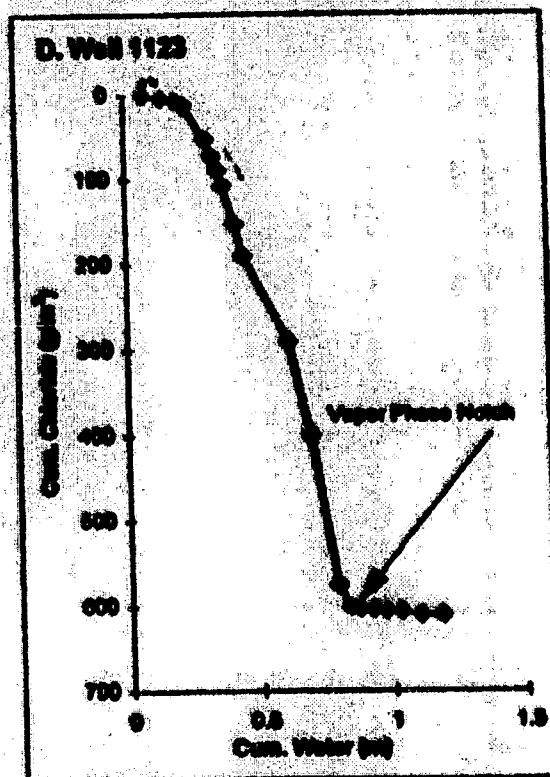
Figure 3. Cumulative water vs. cumulative chloride for wells 1101, 1117, 1121, and 1123.
